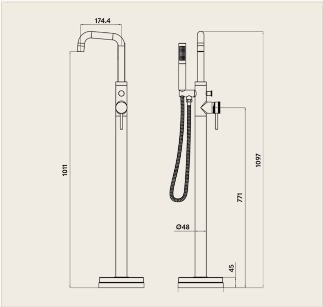
FRONT & SIDE VIEWS • DIMENSIONS IN MM
