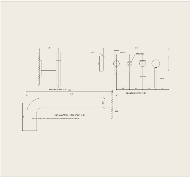
FRONT + SIDE VIEWS • DIMENSIONS IN MM
