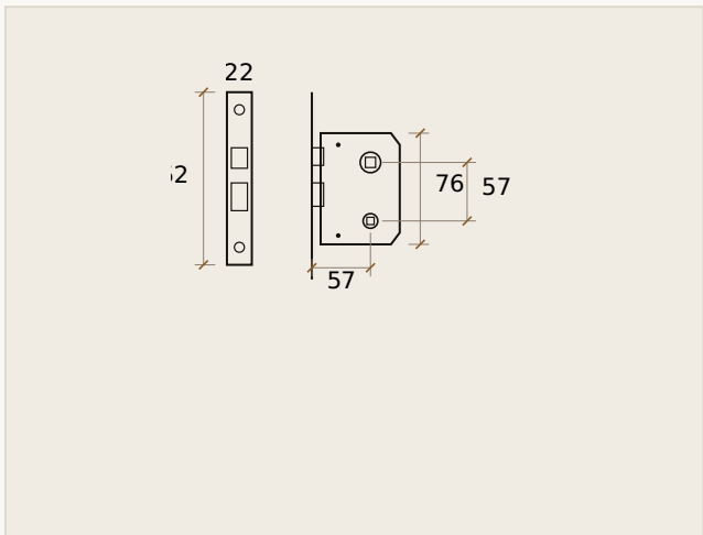
FACE PLATE + CASE PLAN • 1:2 • DIMENSIONS IN MM
