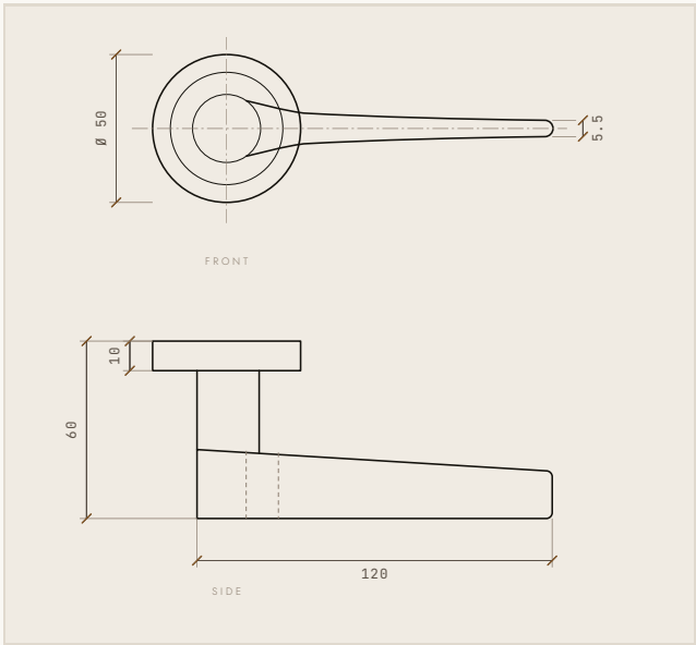
FRONT • SIDE ELEVATION • DIMENSIONS IN MM • DRAWN CAST LONDON
