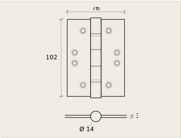
FRONT VIEW • OPEN • 1:2 • DIMENSIONS IN MM
