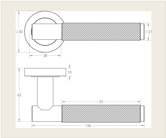
FRONT & PLAN VIEWS • DIMENSIONS IN MM
