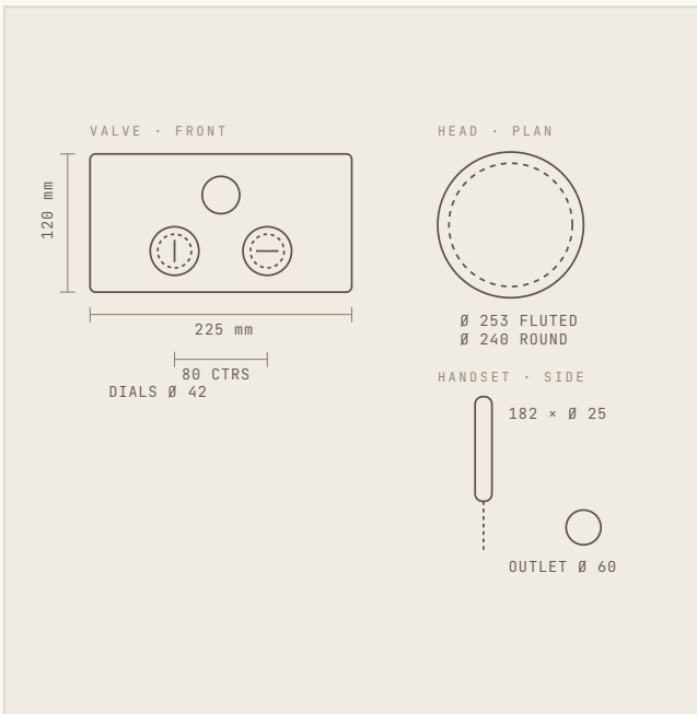
VALVE FRONT • HEAD PLAN • DIMENSIONS IN MM
