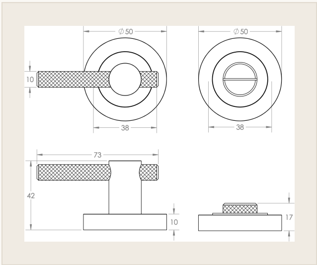
TURN & RELEASE SIDES • DIMENSIONS IN MM
