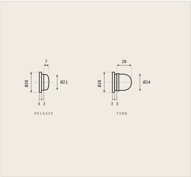
SIDE ELEVATIONS • RELEASE & TURN • DIMENSIONS IN MM
