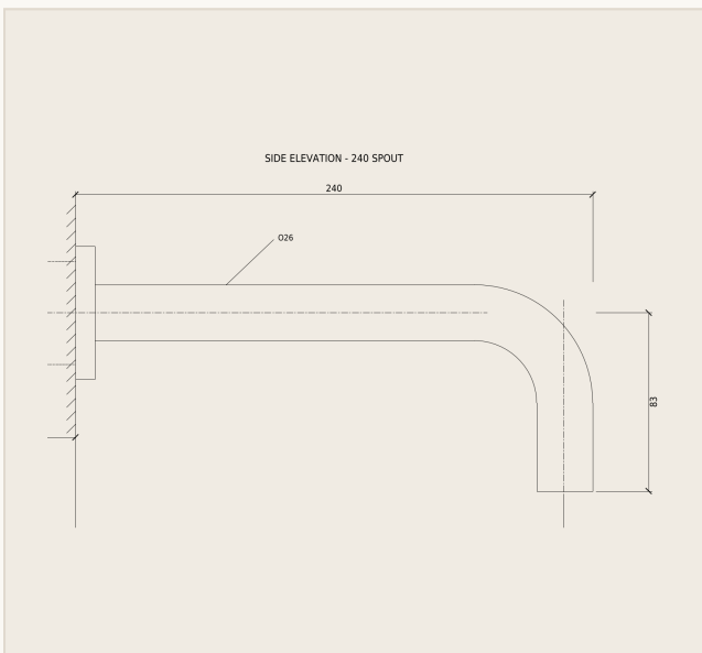
SIDE ELEVATION • 240 SPOUT • DIMENSIONS IN MM • FULL GA: CL-CAD_WB-002 (DXF)
